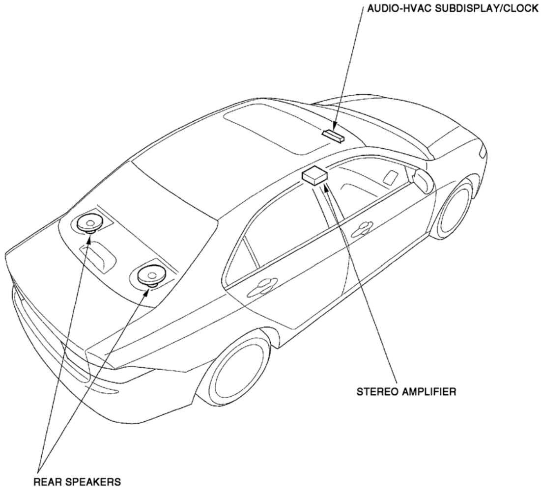
Fig. 2: Locating Audio System Components (2 Of 2)
